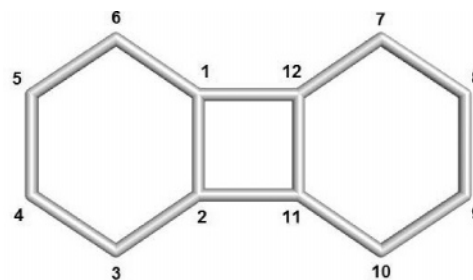
Figure 1. Diphenylene DPH and its numbering.
