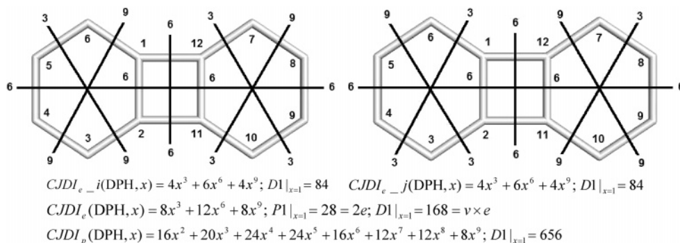
Figure 2. Edge cut procedure for calculating Cluj polynomial CJDI_e in diphenylene DPH.
