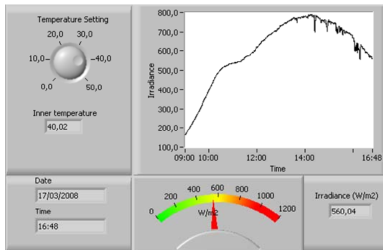
Figure 7. Virtual Instrument (VI) produced to control the pyranometer.
